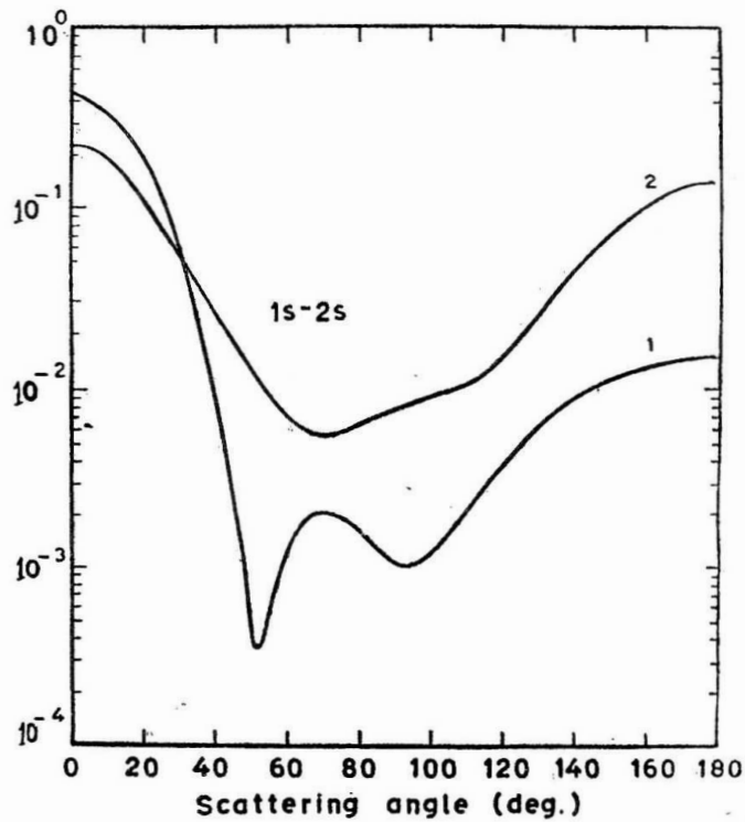
Fig. 1. Differential cross sections ( a_0^2 Sr^{-1} ) for the inelastic scattering process e^- + H(1s) \rightarrow e^- + H(2s) at an incident energy of 1 Ry. Curve 2 are van de Ree results.
