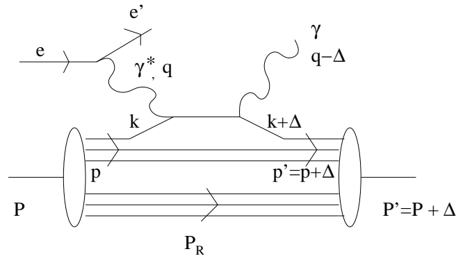
Fig. 1. The DVCS process in the present approach.
