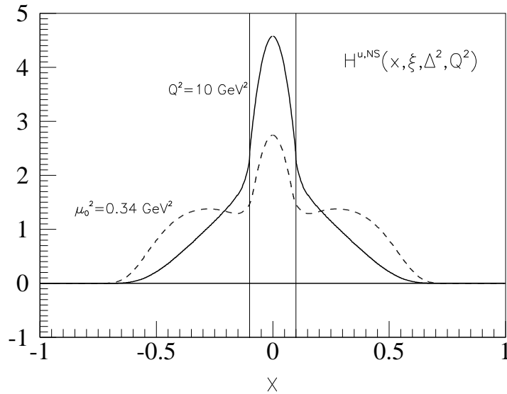
Fig. 3. The NS H GPD for valence u-quarks at \xi = 0.2 and \Delta^2 = -0.5 \text{ GeV}^2 , at the momentum scale of the model, \mu_0^2 = 0.34 \text{ GeV}^2 (dashed), and after NLO-QCD evolution up to Q^2 = 10 \text{ GeV}^2 (full).
